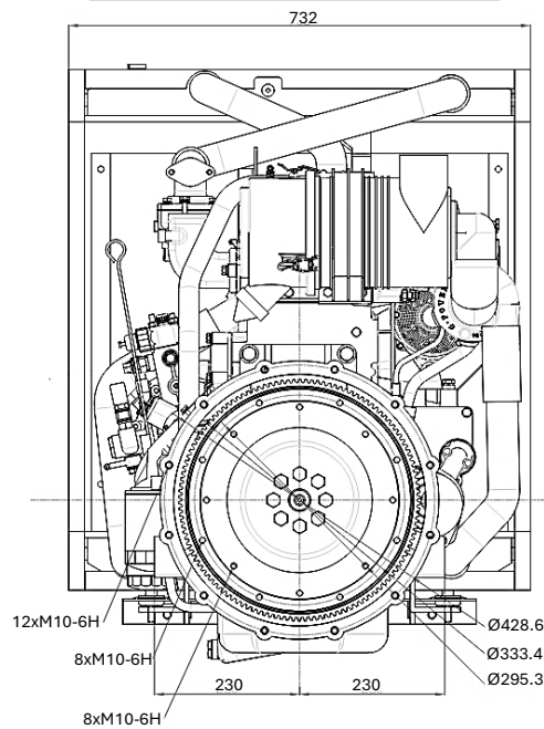
REAR VIEW - FLYWHEEL
