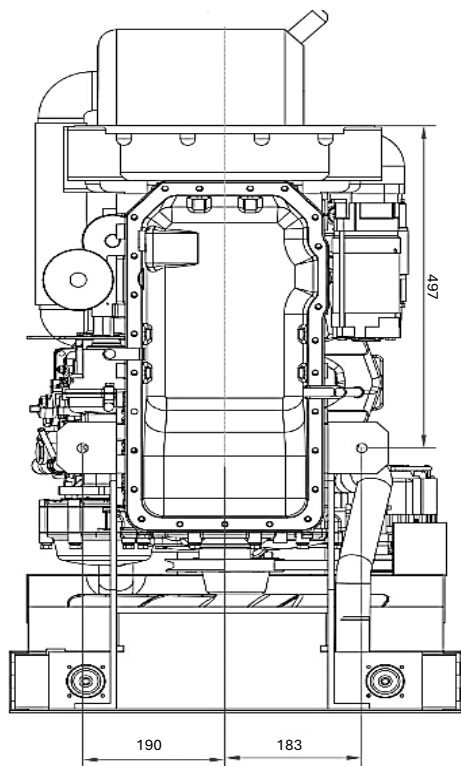
BOTTOM VIEW - LOW
