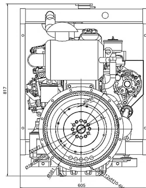
REAR VIEW - FLYWHEEL
