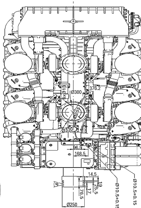
TOP VIEW - AERIAL
