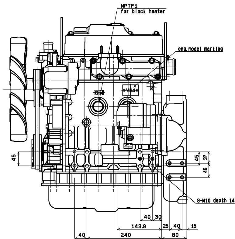
Starter side
