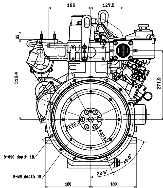
Flywheel side
