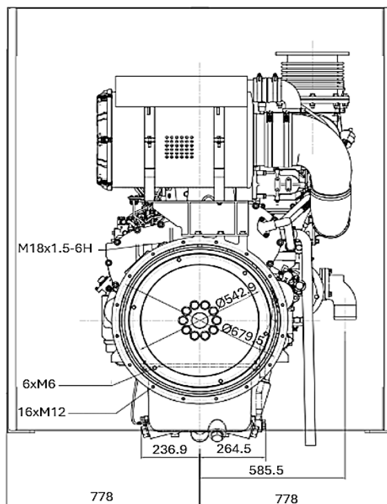
REAR VIEW - FLYWHEEL
