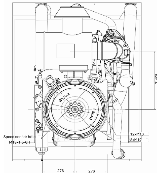
REAR VIEW - FLYWHEEL
