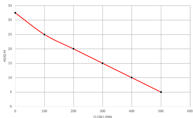
PERFORMANCE CURVE
