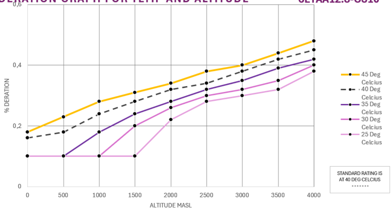
DERATION GRAPH FOR TEMP AND ALTITUDE
