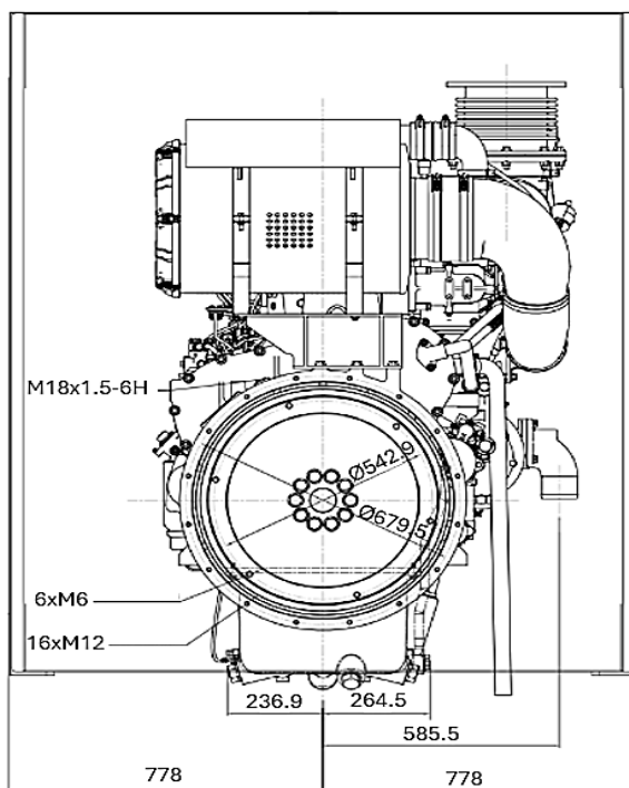
REAR VIEW - FLYWHEEL
