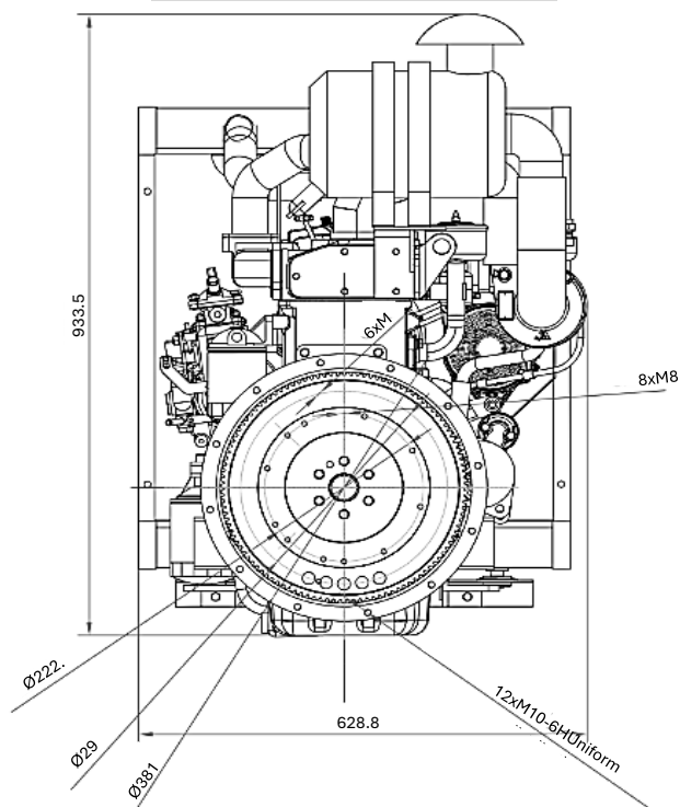
REAR VIEW - FLYWHEEL
