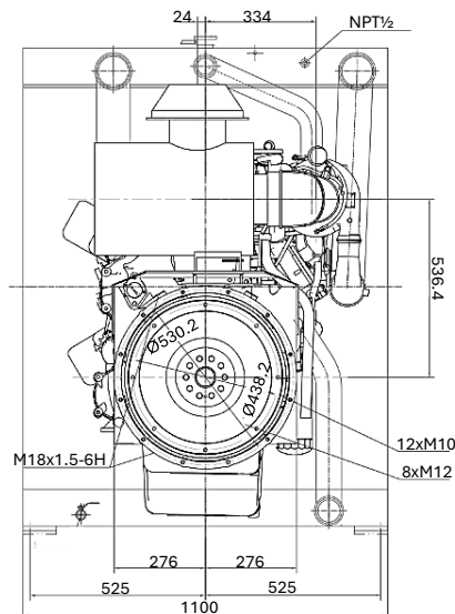
REAR VIEW - FLYWHEEL
