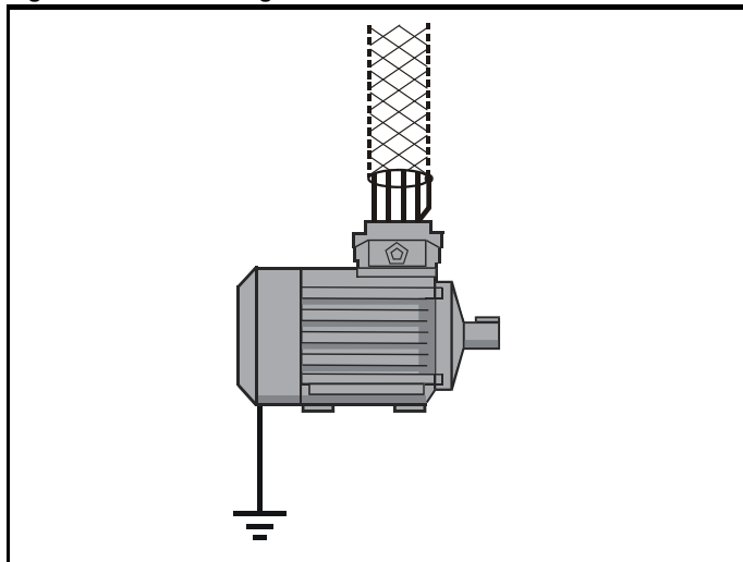
Figure 4-42 Grounding the motor cable shield
