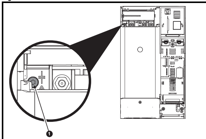
Figure 4-32 Removal of the size 6 internal EMC filter
