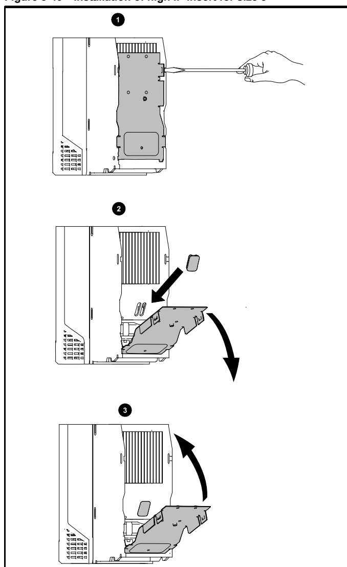
Figure 3-40 Installation of high IP insert for size 3
