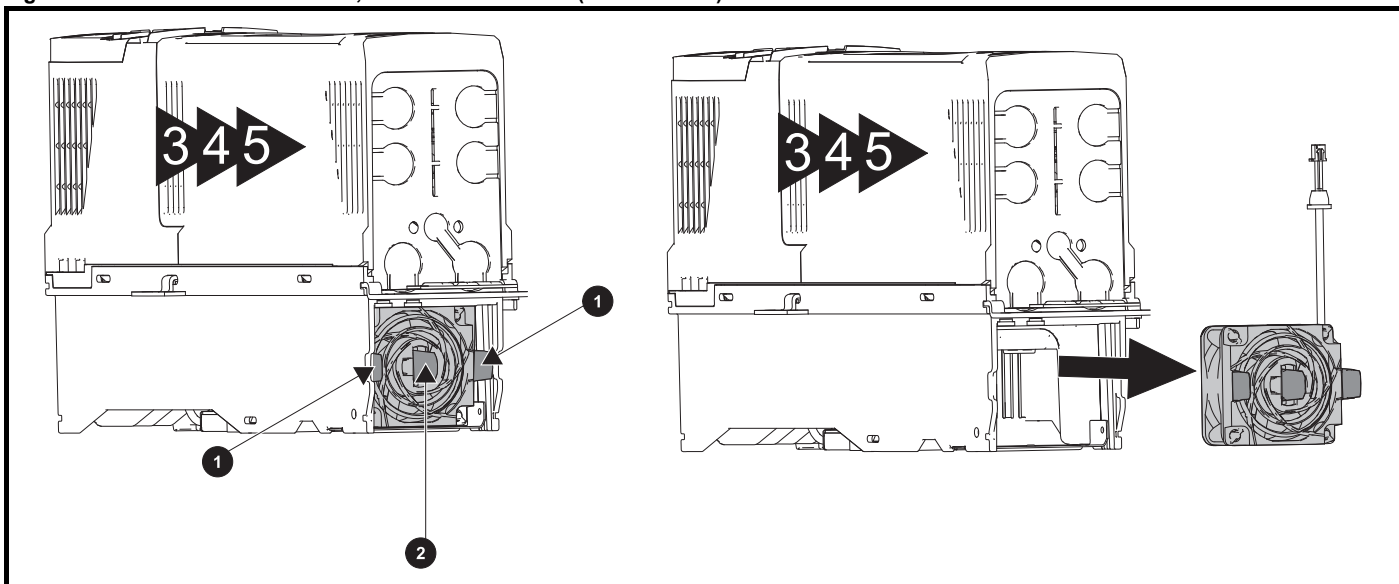
Figure 3-64 Removal of the size 3, 4 and 5 heatsink fan (size 3 shown)
