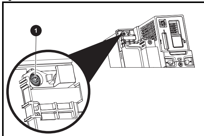
Figure 4-30 Removal of the size 4 internal EMC filter
