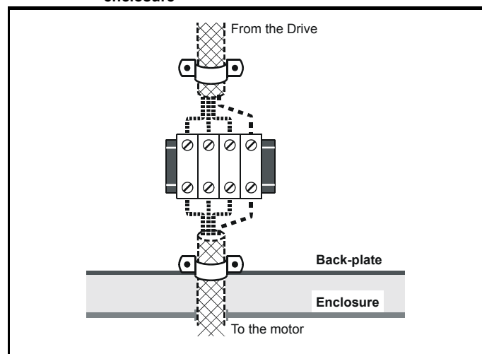
Figure 4-44 Connecting the motor cable to a terminal block in the enclosure
