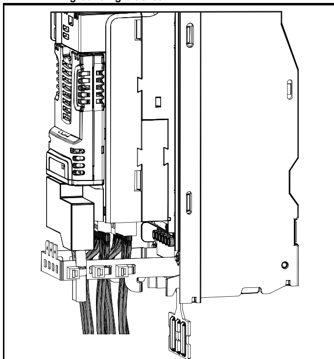
Figure 4-43 Grounding of signal cable shields using the grounding bracket
