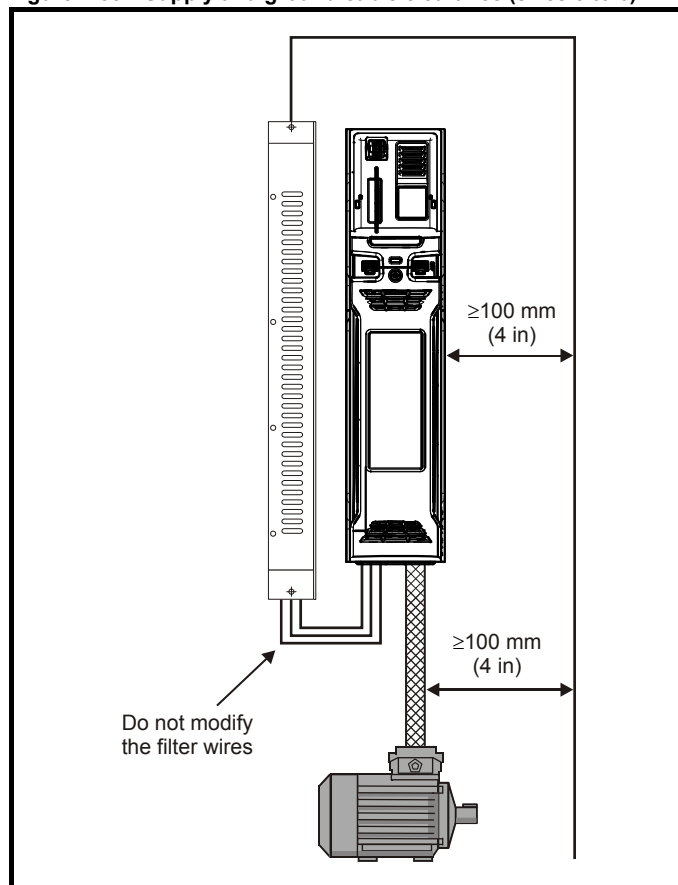
Figure 4-38 Supply and ground cable clearance (sizes 3 to 6)
