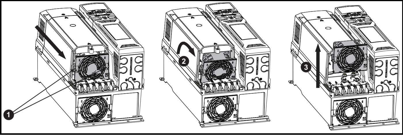
Figure 3-69 Removal of the size 6 auxiliary(capacitor bank) fan
