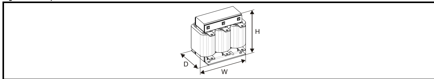
Figure 4-14 Input line reactor dimensions
