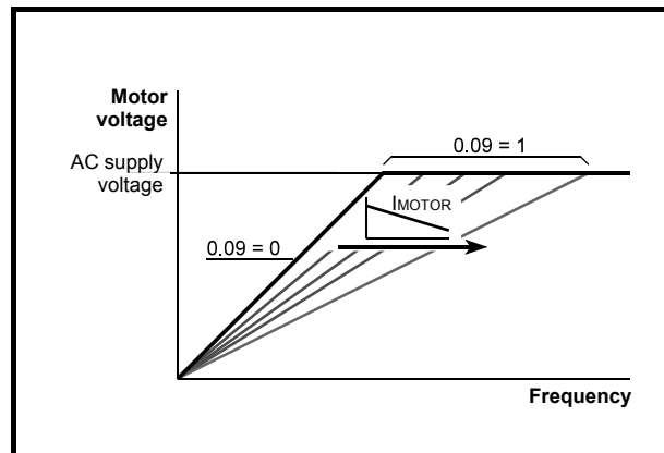
Figure 6-2 Fixed and variable V/f characteristics
