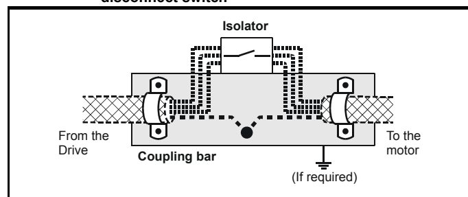
Figure 4-45 Connecting the motor cable to an isolator / disconnect switch
