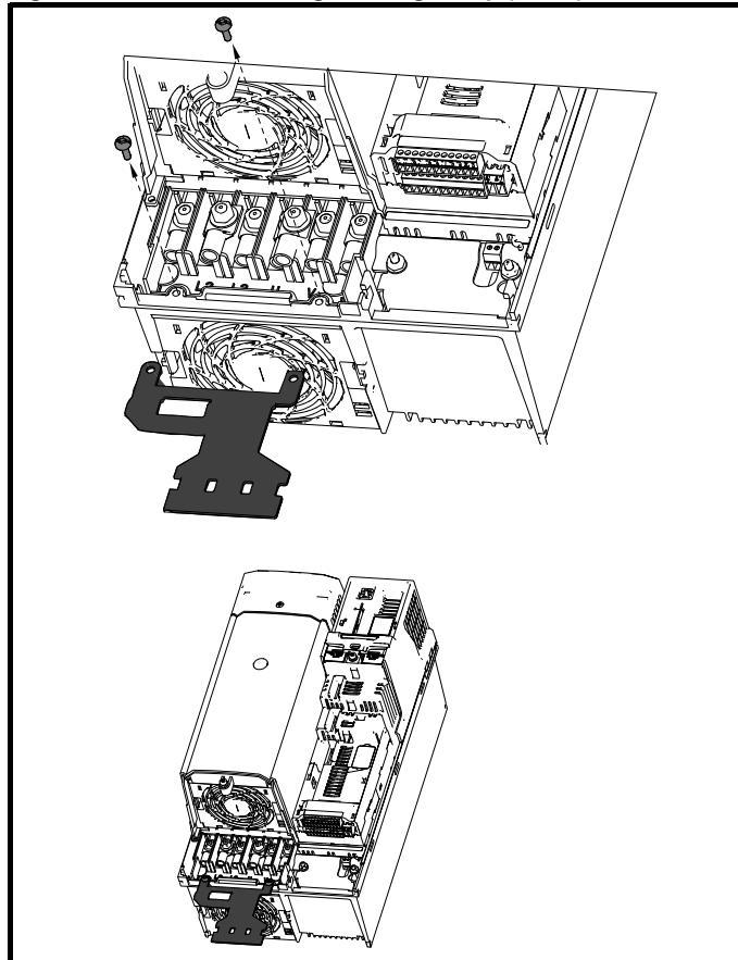
Figure 4-27 Installation of grounding clamp (size 6)
