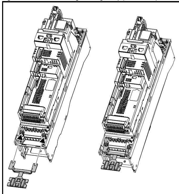
Figure 4-25 Installation of grounding clamp (size 3 and 4)
