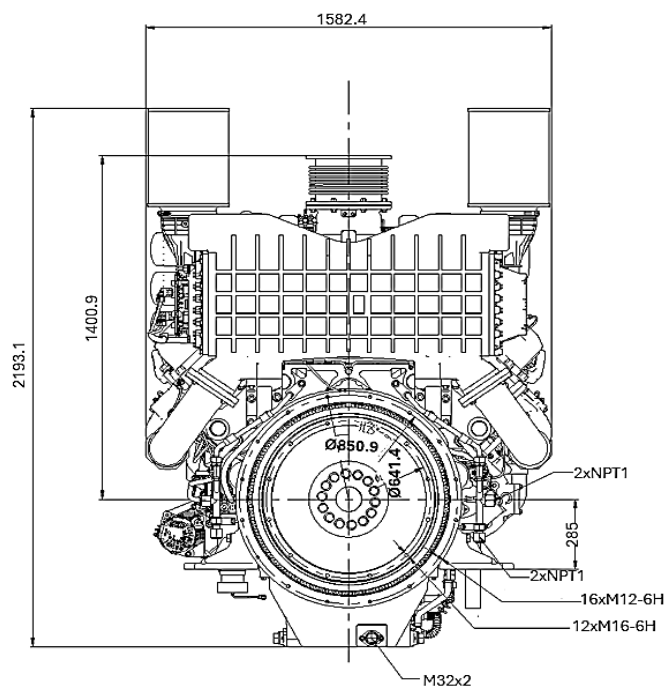
REAR VIEW - FLYWHEEL
