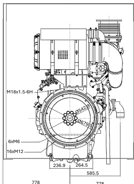
REAR VIEW - FLYWHEEL
