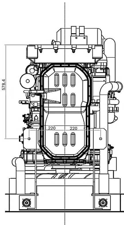
BOTTOM VIEW - LOW
