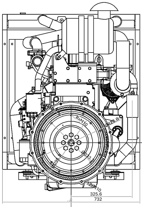
REAR VIEW - FLYWHEEL
