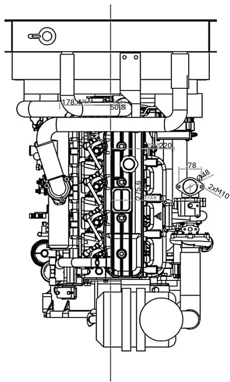
REAR VIEW - FLYWHEEL
