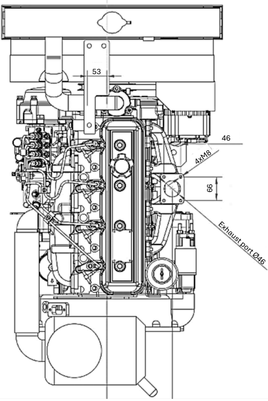
REAR VIEW - FLYWHEEL
