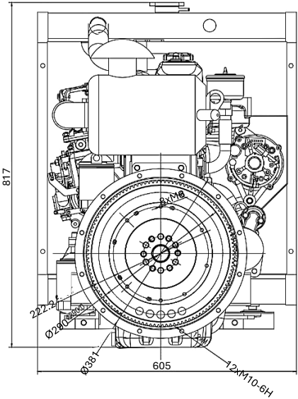
REAR VIEW - FLYWHEEL
