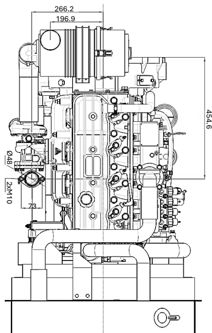
TOP VIEW - AERIAL
