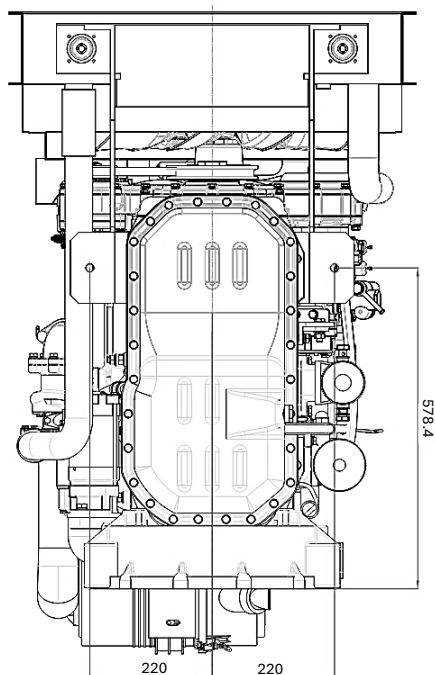
BOTTOM VIEW - LOW
