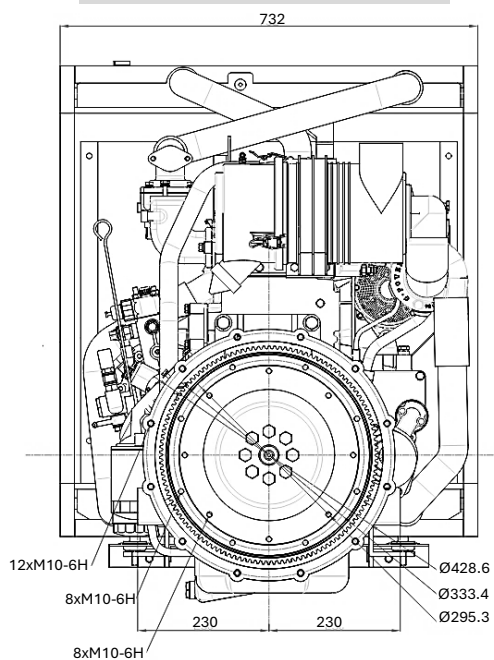
REAR VIEW - FLYWHEEL
