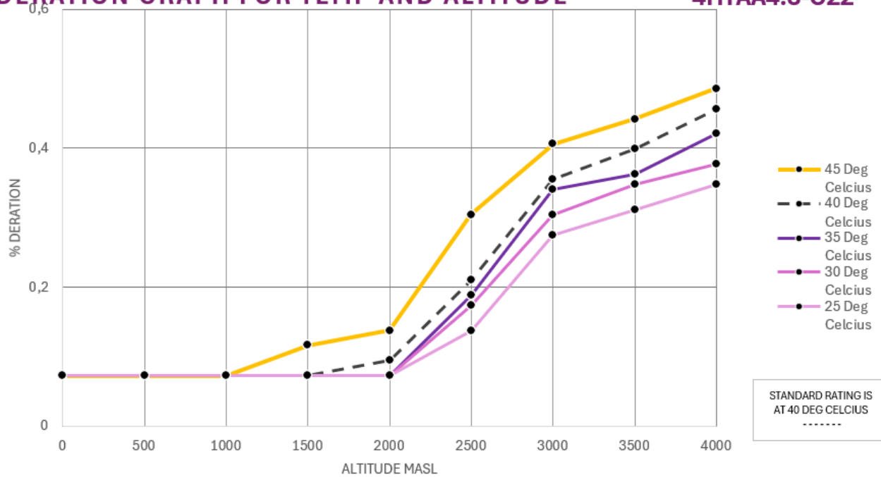
DERATION GRAPH FOR TEMP AND ALTITUDE
