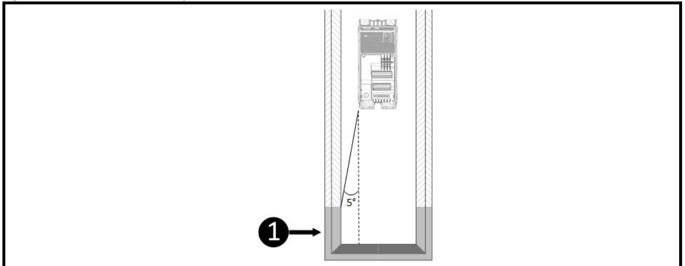
Figure 3-1 Fire enclosure bottom layout
