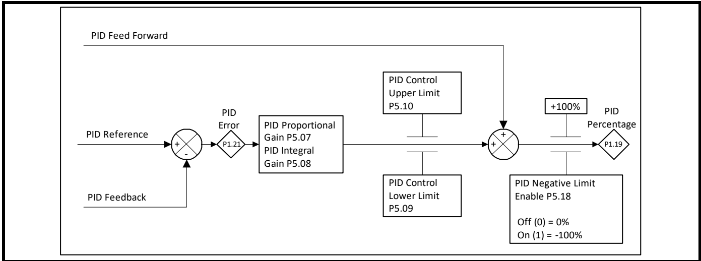
Figure 7-14 PID controller overview
