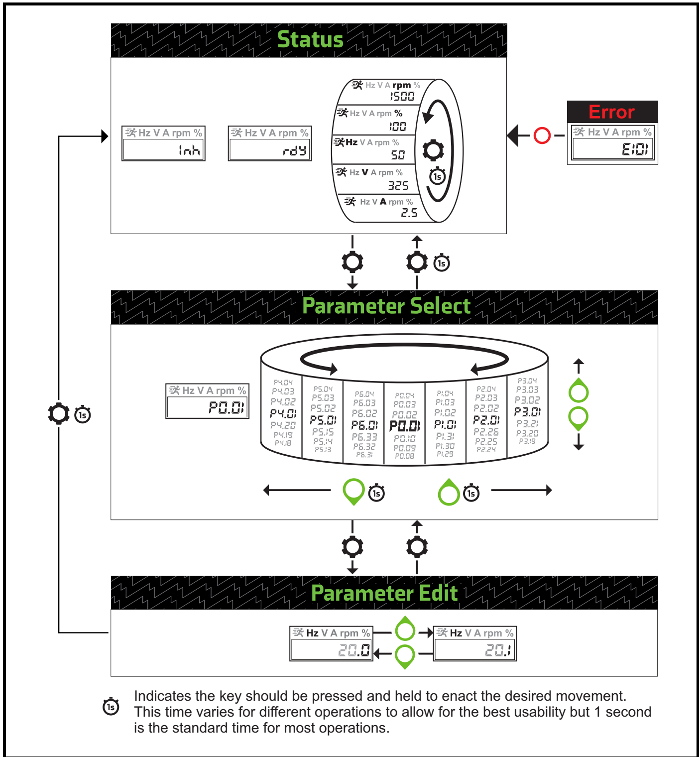
Figure 5-4 Menu structure
