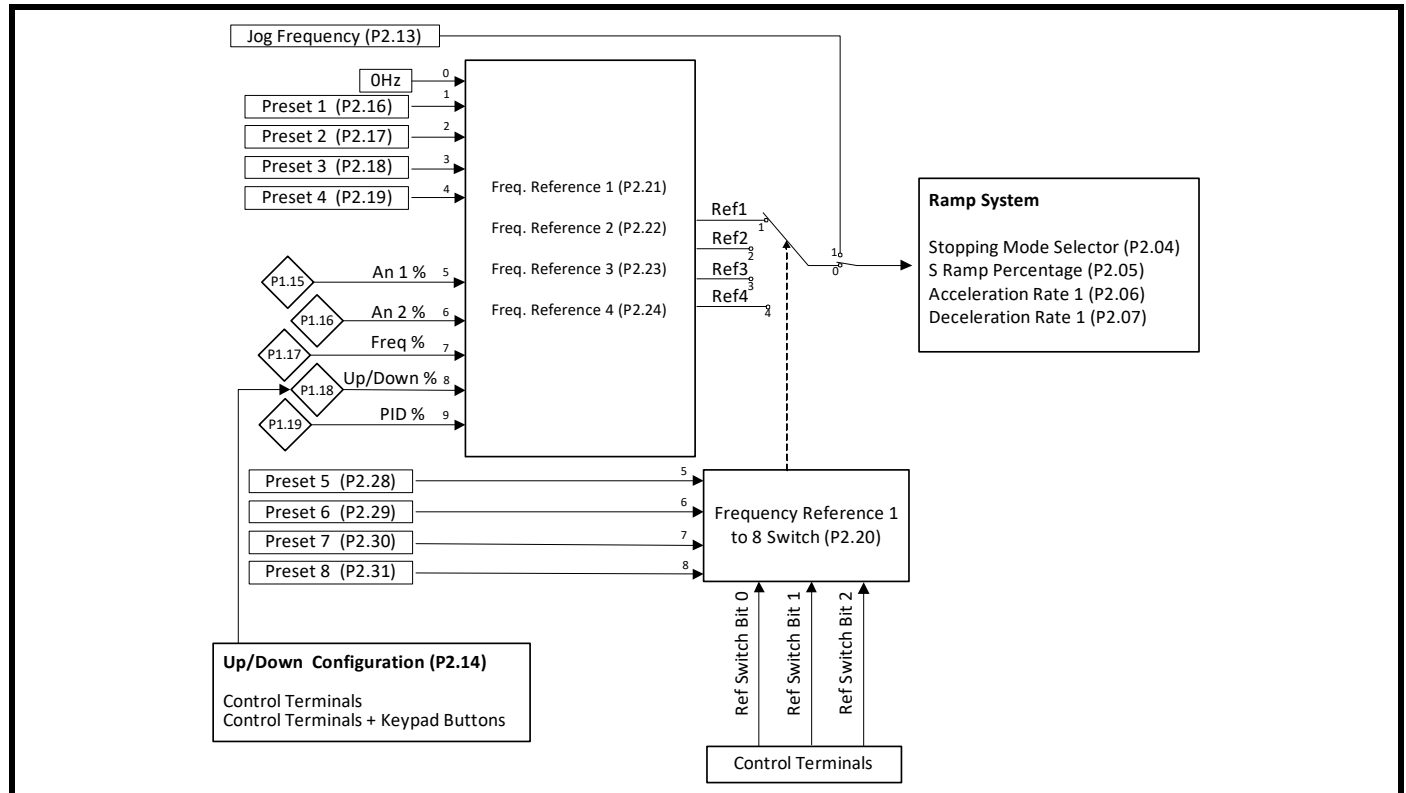
Figure 7-2 Menu 2 - Reference & ramps
