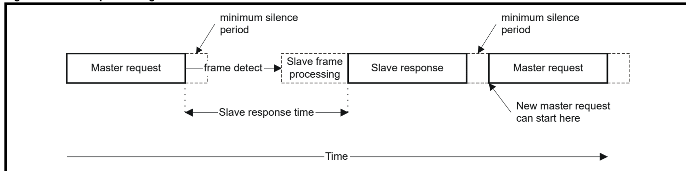
Figure 8-2 Frame processing
