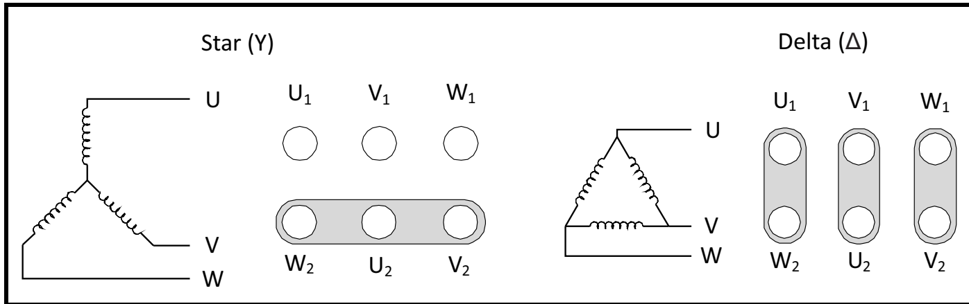
Figure 4-5 Typical \Delta / \Delta connections in a motor
