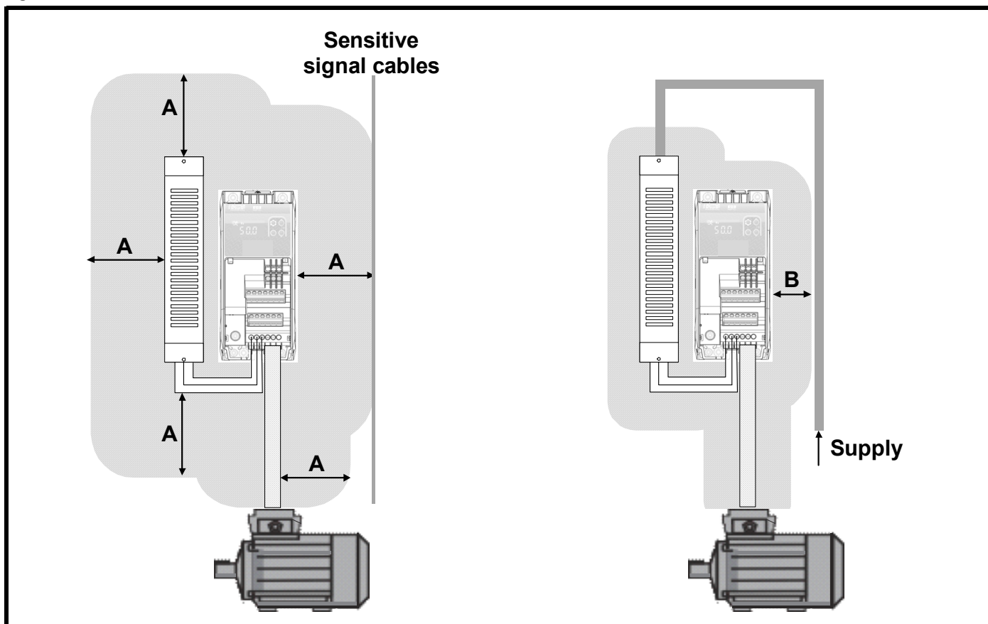
Figure 4-9 Suitable cable clearances
