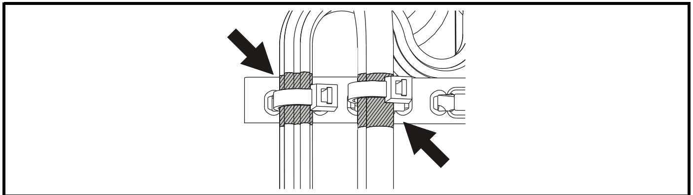
Figure 4-8 Grounding the motor cable shield
