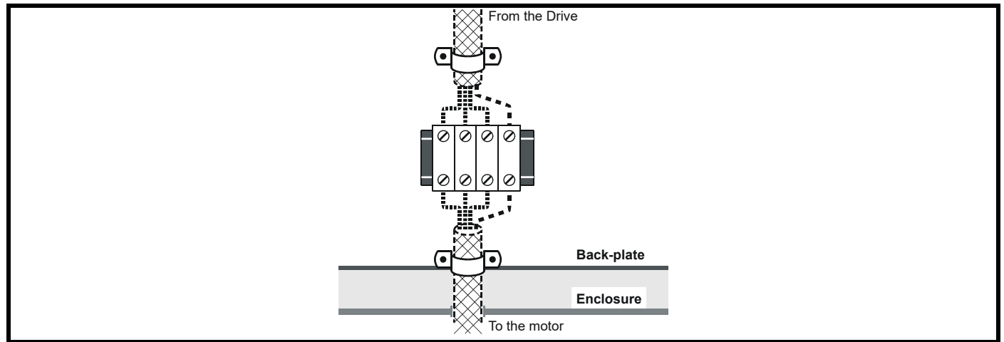
Figure 4-10 Connecting the motor cable to a terminal block in the enclosure
