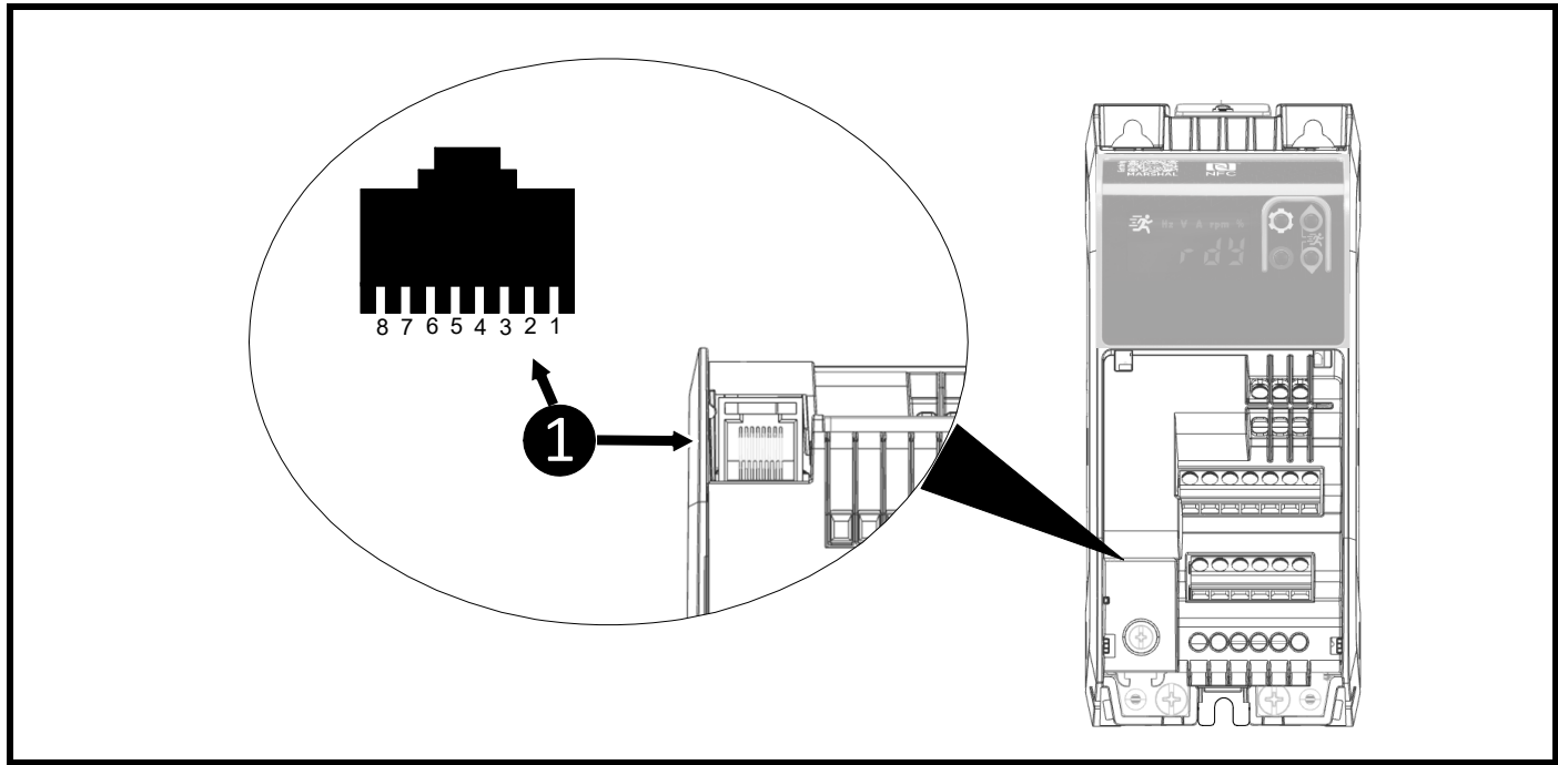
Figure 4-15 Location of the 485 serial communications port
